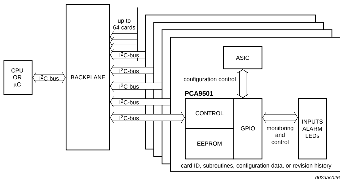
Fig 21. PCA9501 used as interface for board configuration
